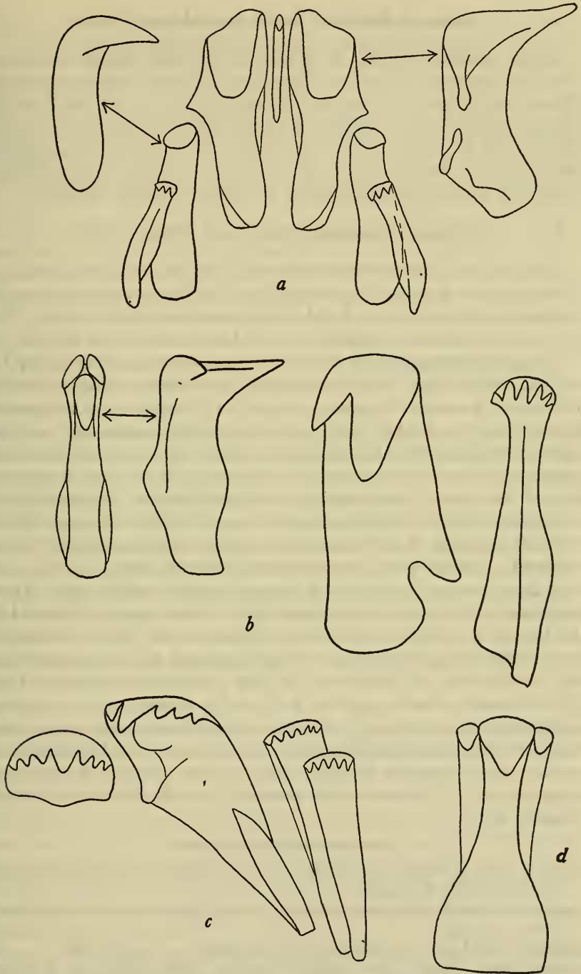
FIGURE 57.—Radulae of, a , Echininus nodulosus Pfeiffer, b , Nodilittorina tuberculata Menke, c , Modulus modulus Linné, and, d , the central tooth of Tectarius muricatus Linné. (Arrows point to side views of teeth.)
